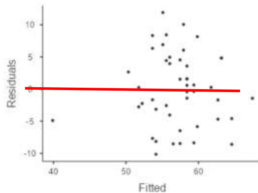
Gambar 2. Residual Plot: Psychological Capital dan Work Engagement
