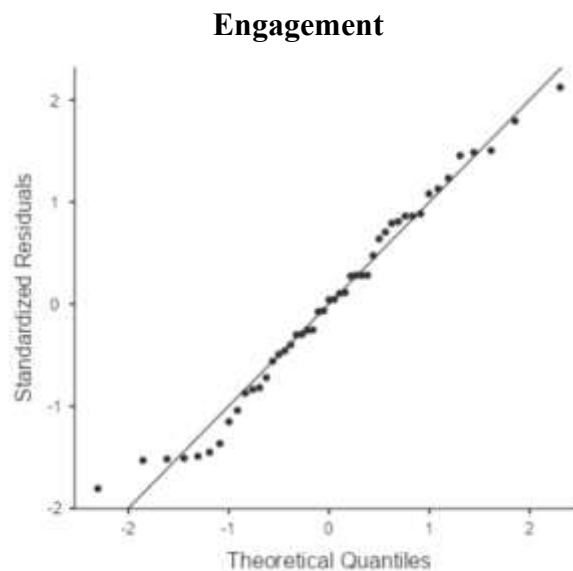
Gambar 1. Q-Q Plot Standardized Residuals: Psychological Capital dan Work
